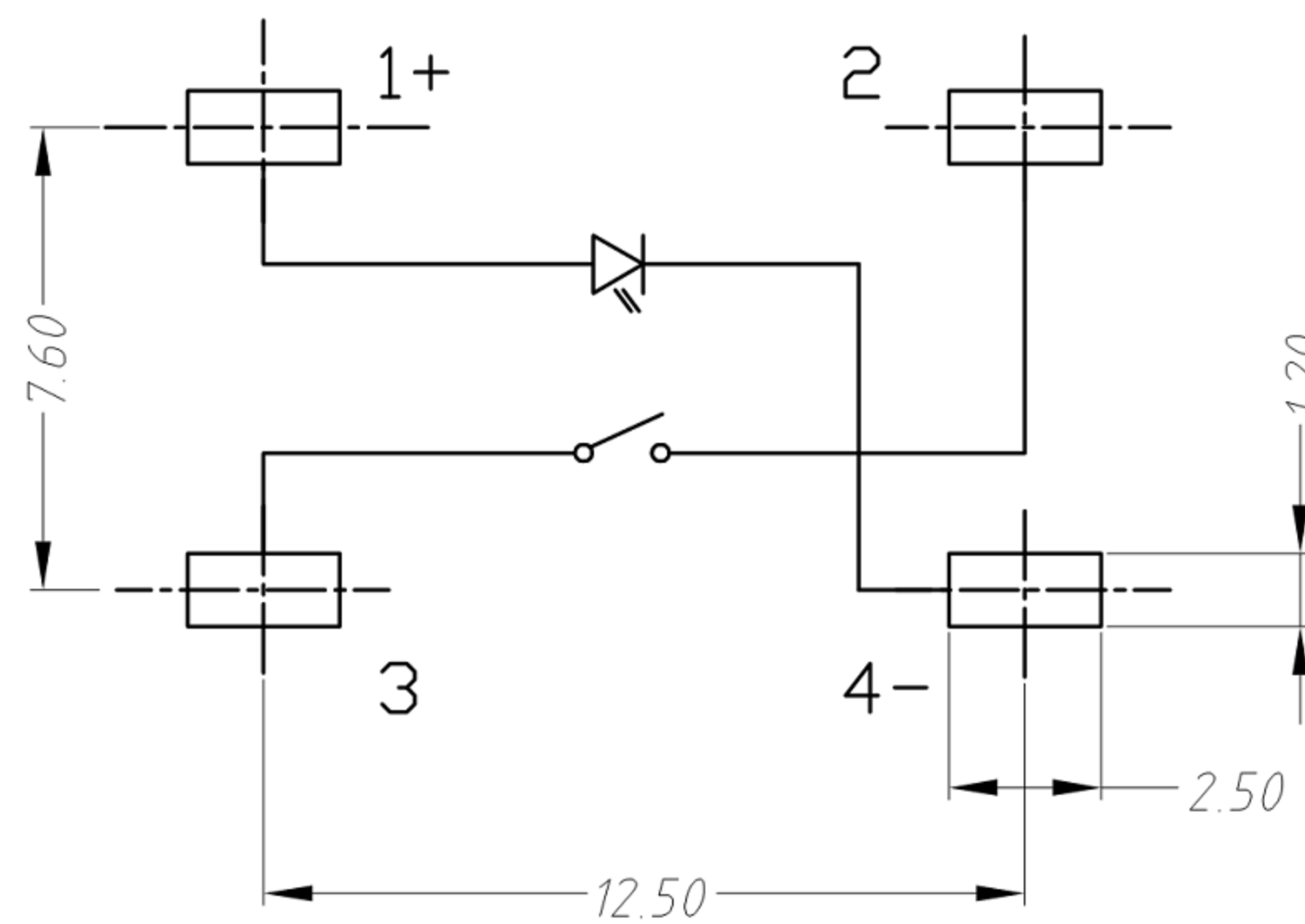
PCB layout and Circuit Diagram
